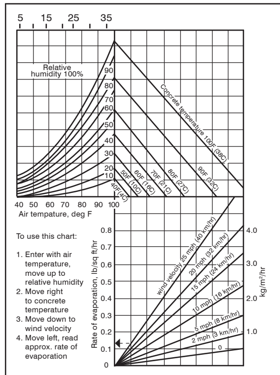
Fig. 2.1.5, ACI 305, Hot Weather Concreting
